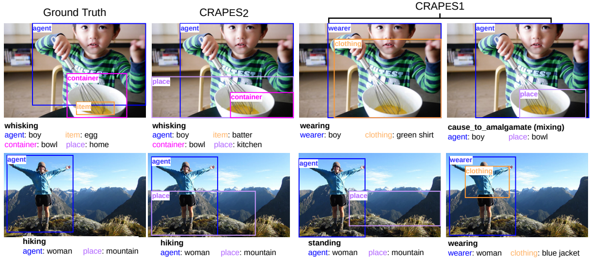
Figure 5: Examples of predictions made by CRAPES. The first column lists the GT image and frame from the SWiG test set. The second column lists the prediction from CRAPES 2 (V+L and SRL parser trained on SWiG). Last two columns depicts parallel frames detected by CRAPES 1 (V+L trained on Flickr30k and LOME parser)
